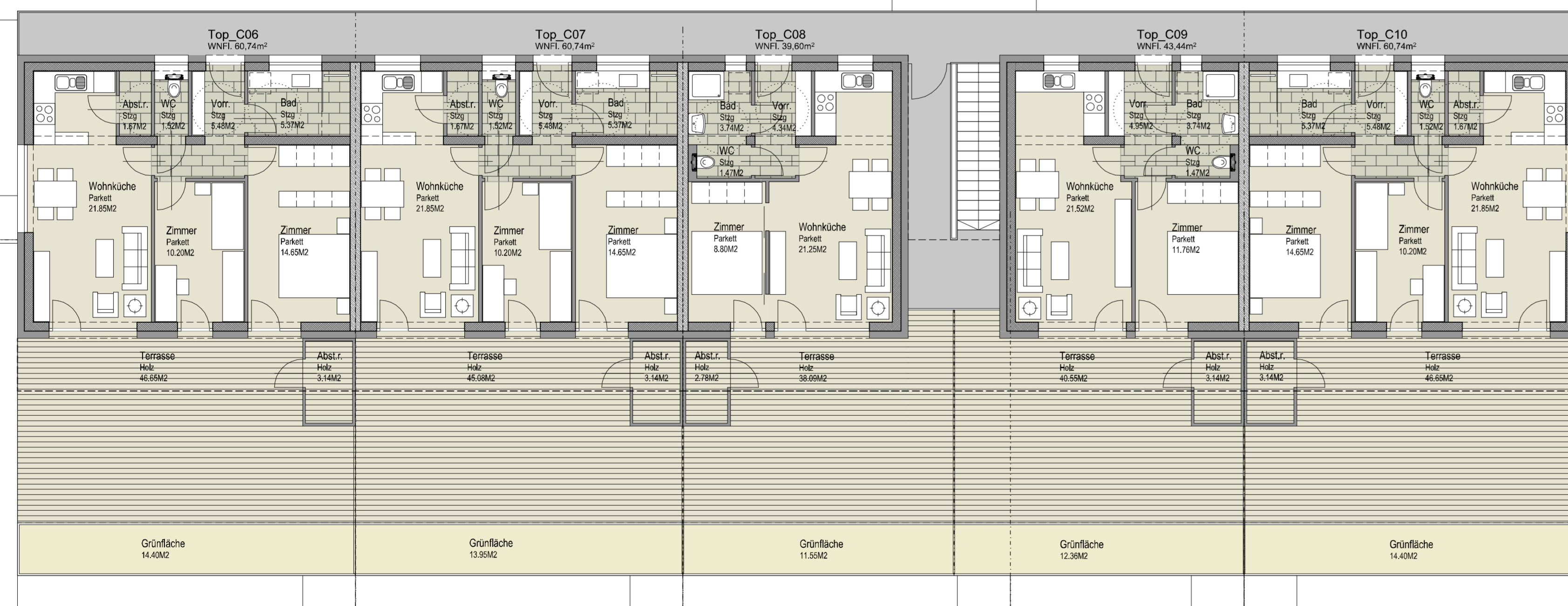
HAUS C WNFL 1.OG : 285,26m 2
